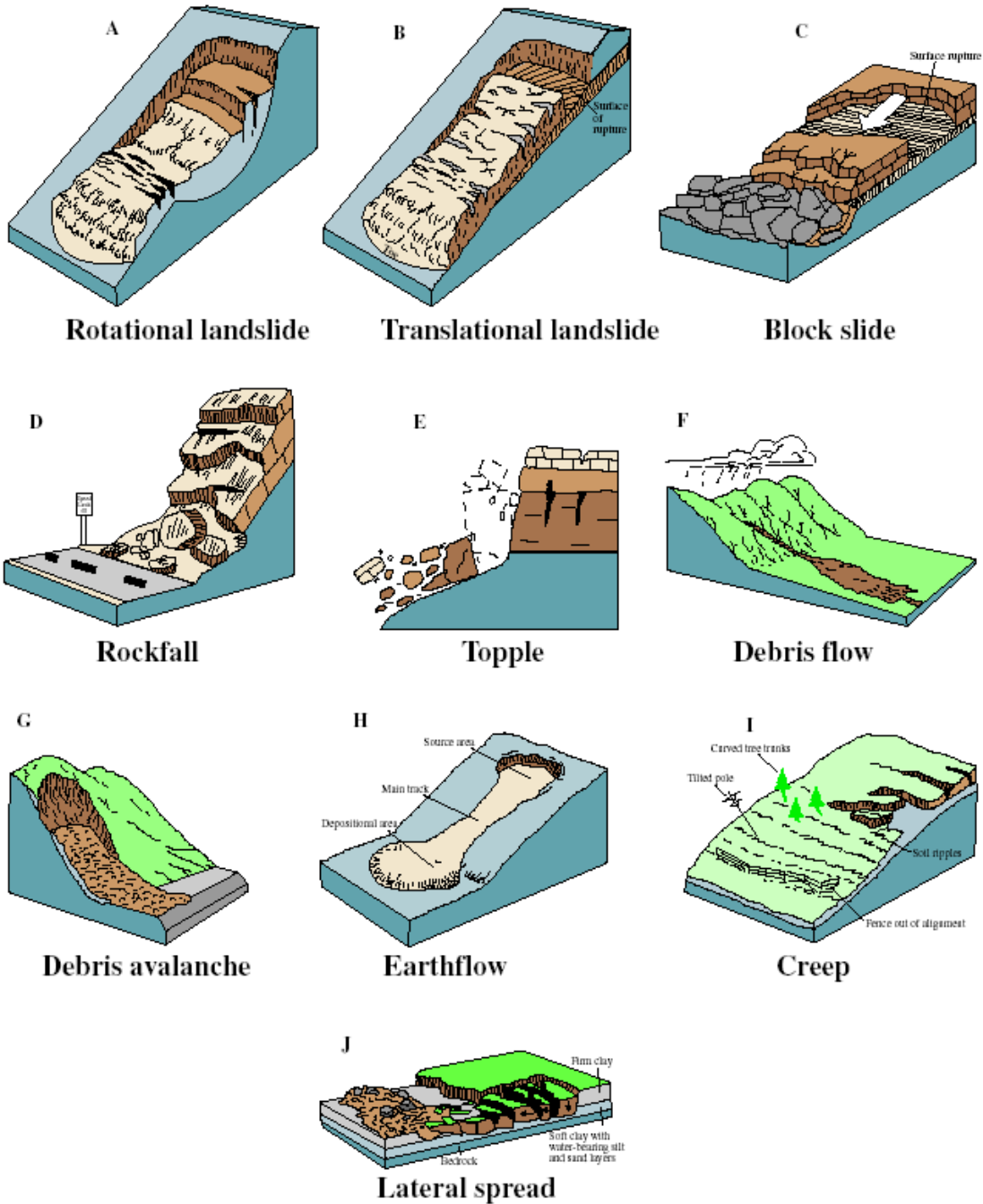
Figure 7-1 Landslide Types
